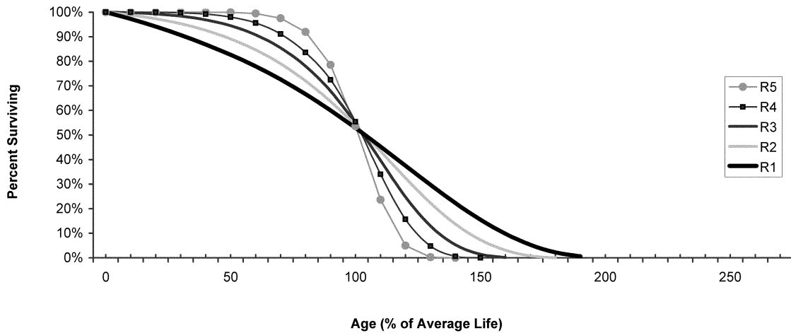
Figure 3 Iowa R Family Survivor Curves
